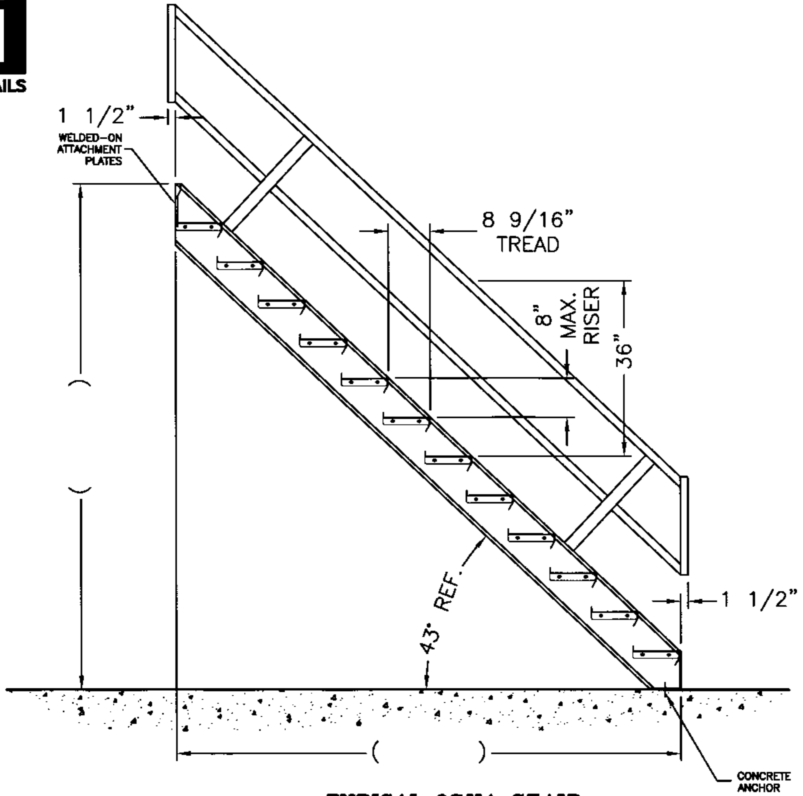
TYPICAL OSHA STAIR (2-RAIL STANDARD)
