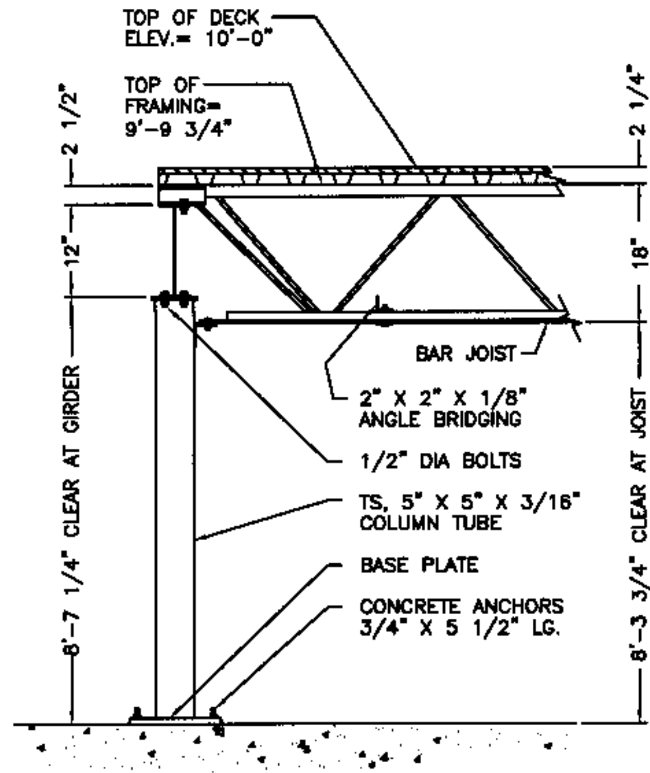
TYPICAL SECTION AT COLUMN
