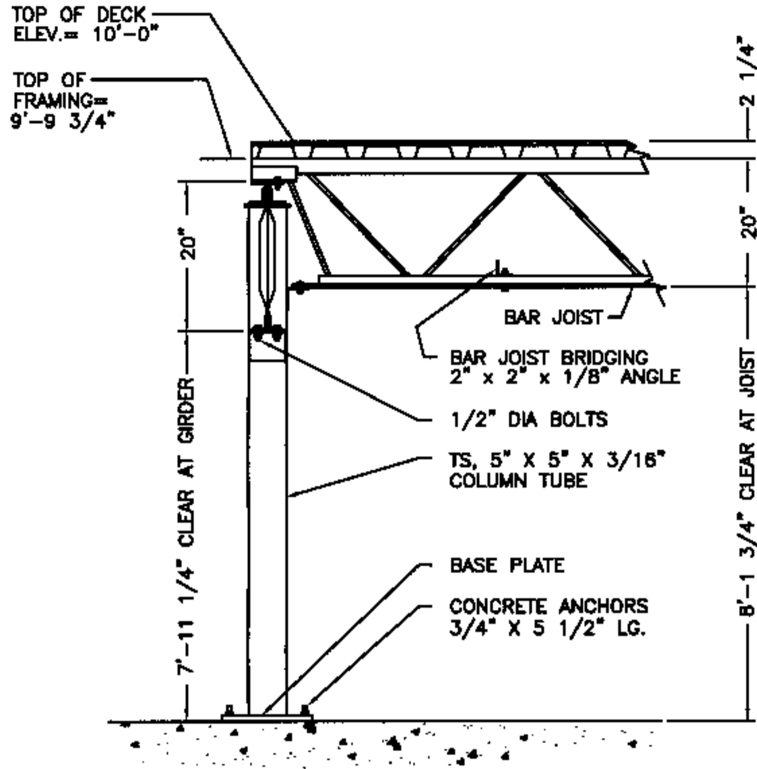
TYPICAL SECTION AT COLUMN
